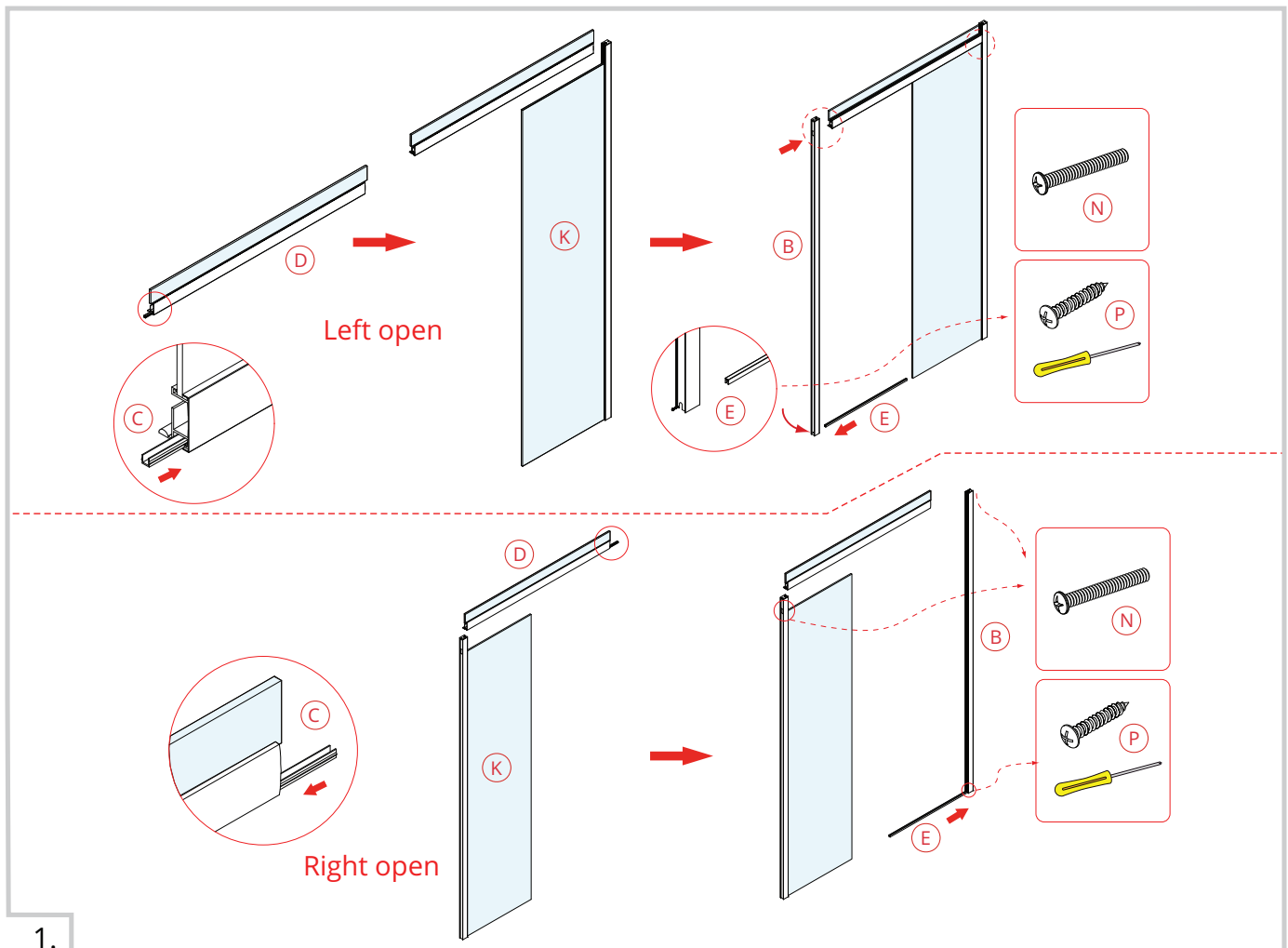
Parts List
